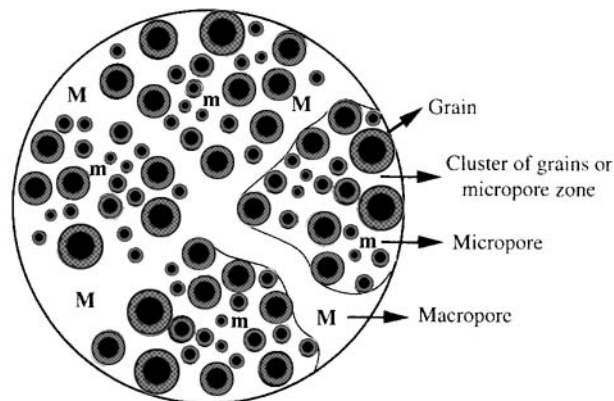
Figure 1. Calcined limestone particle according to the grain model of Szekely and Evans (1970).
